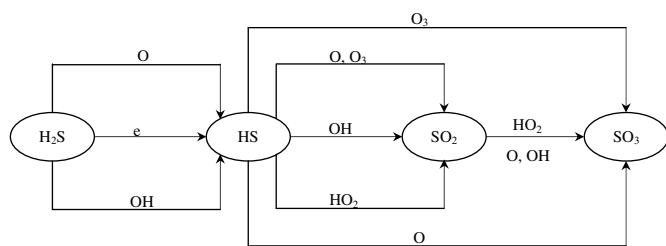
Fig. 13. Dominant pathways leading to the destruction of \text{H}_2\text{S} molecules.
