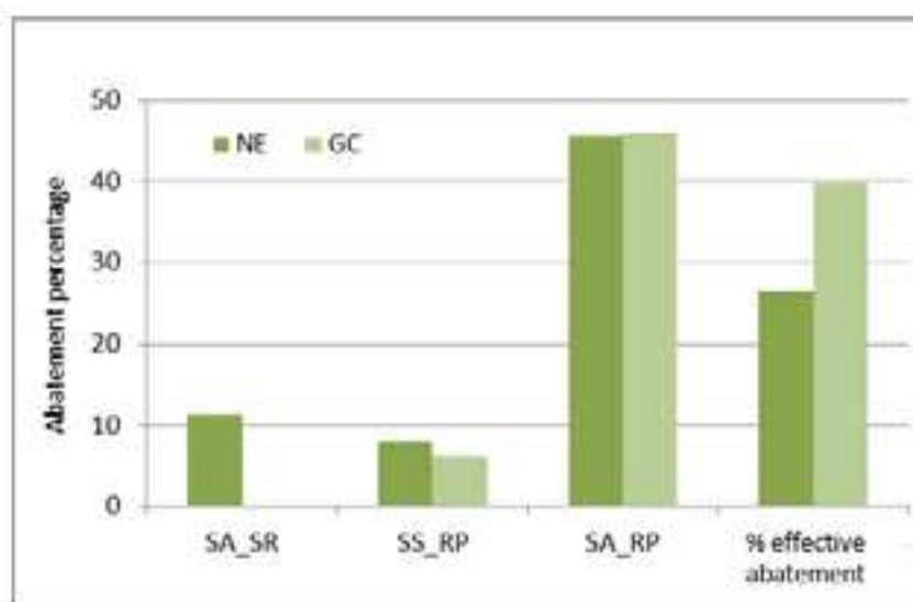
Figure 28. Results of tests conducted on LA waste expressed as abatement percentages, taken at the sampling points 1 and 3.
