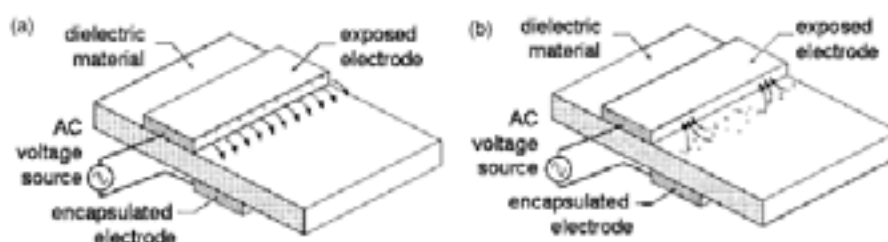
Figure 3 – DBD functioning: (a) negative semi-cycle and (b) positive semi-cycle
