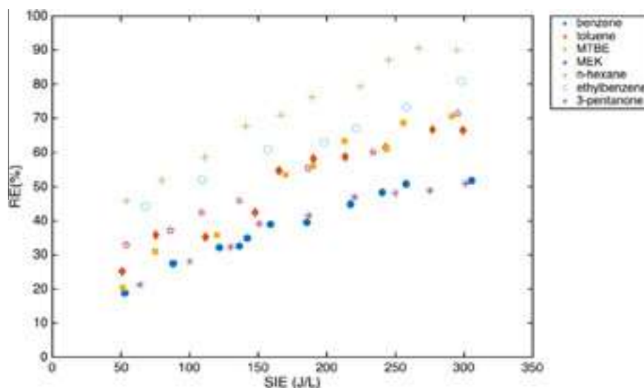
Fig. 2. Removal efficiencies (REs) of selected VOCs as a function of applied specific input energy (SIE) for a flow rate of 6.6 \text{ L min}^{-1} and an inlet VOCs concentration of 95 \text{ ppm}_v .
