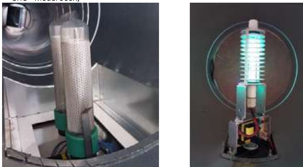
Picture 1 - JONIX-NTP (left), SHU 900X (right)
