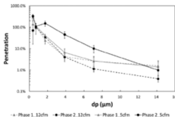
Fig. 3. Penetration of particles (downstream number concentration / upstream number concentration) in each OPC size bin measured at two flow rates in the two test program phases.
