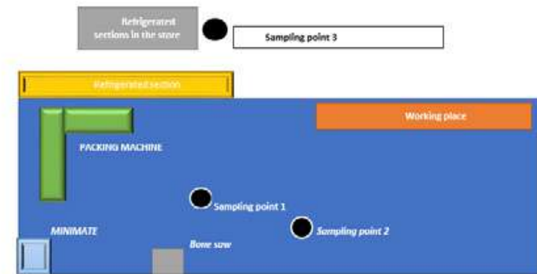
Figure 1. Plan view of the room Dimensions: 15 \times 5 \times 4 \text{ m} = 75 \text{ m}^2 - 300 mc. Open side towards the store, dimensions mt. 13 x 2.5 approx. 32.5 \text{ m}^2 open area. The result is an air volume mix of approx. 30,904 \text{ m}^3/\text{h} .
