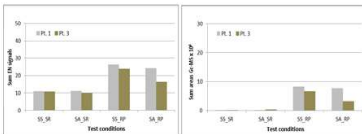
Figure 27. Results of tests conducted on MIX mixed waste (EN left; GC-MS right).
