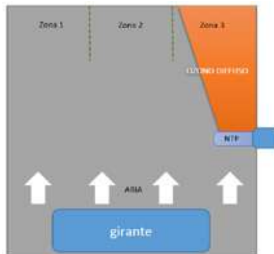
Figure 15 - hypothesis regarding ozone diffusion inside the fan coil
