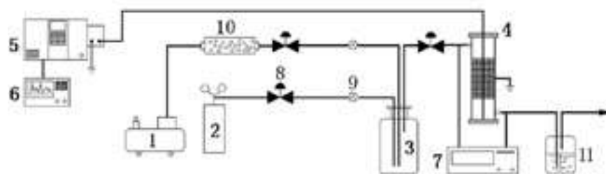
Fig. 1. Schematic diagram of the experimental setup 1. Air compressor 2. \text{H}_2\text{S} gas cylinder 3. Mixing chamber 4. DBD reactor 5. AC power supply 6. Oscilloscope 7. Spectrophotometer 8. MFC 9. Needle valve 10. Gas filtration system 11. Absorbent.
