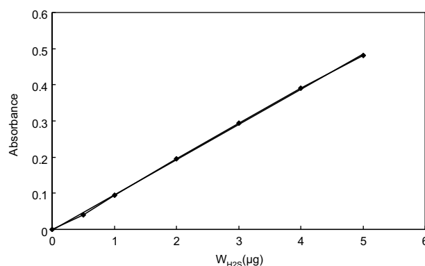
Fig. 2. Typical standard curve for light absorbance with the mass of \text{H}_2\text{S} .
