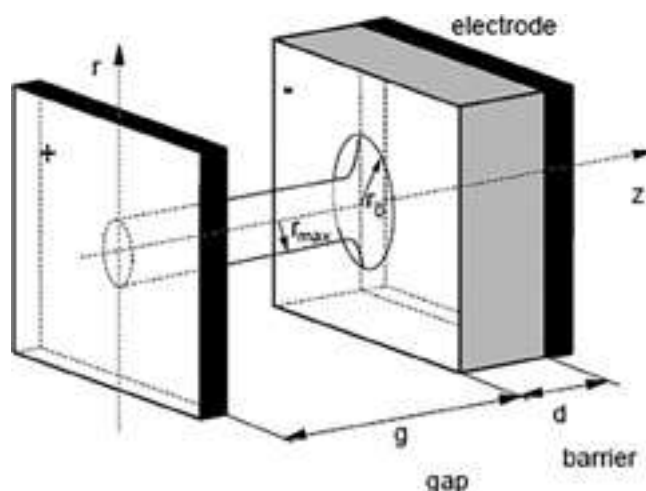
Fig. 5. The shape of a single microdischarge [64].
