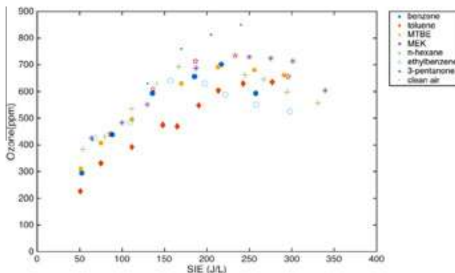
Fig. 4. SIE impact on effluent ozone concentration at a flow rate of 6.6 \text{ L min}^{-1} . Typical standard deviations for the ozone measurements were 40–60 ppm v .
