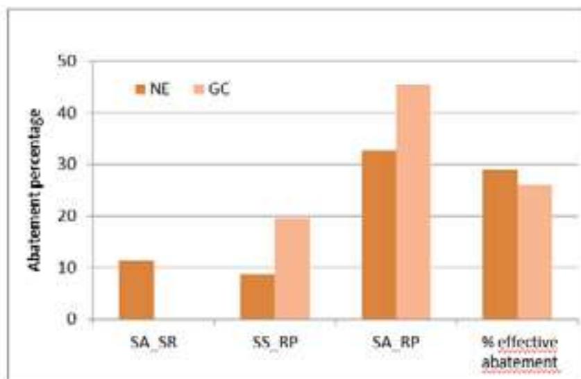
Figure 28. Results of tests conducted on MIX waste expressed as abatement percentages, taken at the sampling points 1 and 3. Legenda: SA_SR = % probe contribution; SS_RP = % decrease due to waste emission losses along the way; SA_RP = % abatement incorrect probe; % effective abatement = SA_RP – SS_RP – SA_SR
