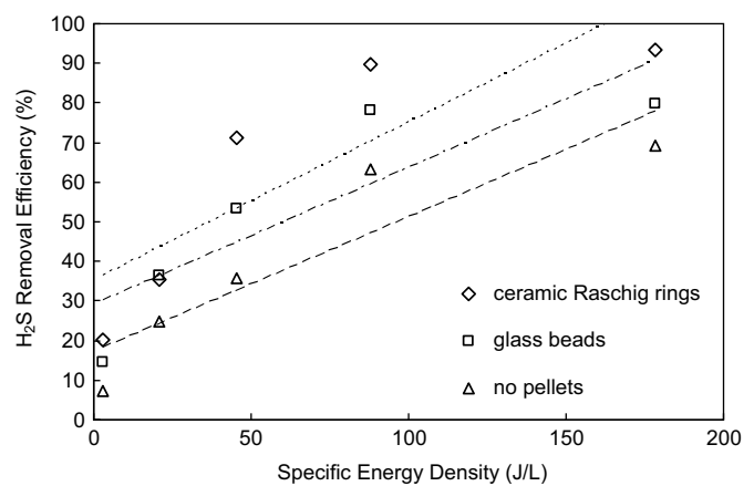
Fig. 12. Relationship between \eta and SED and linear fits for different reactors.
