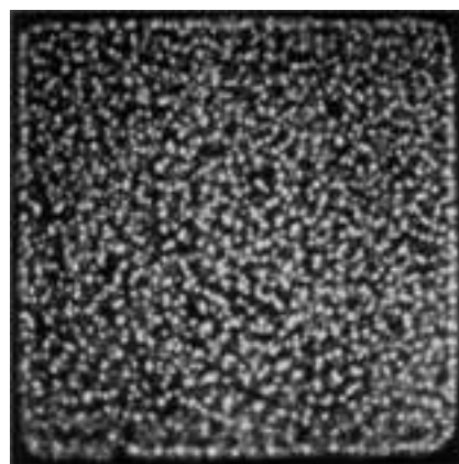
Fig. 4. End-on view of microdischarges in atmospheric-pressure air [51].
